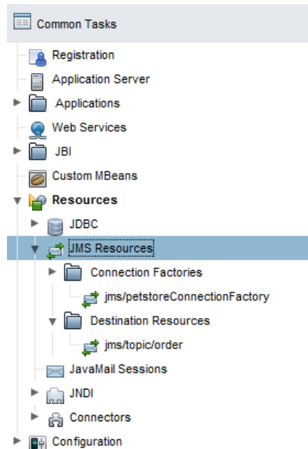
Figure 5-8: JMS Resources
