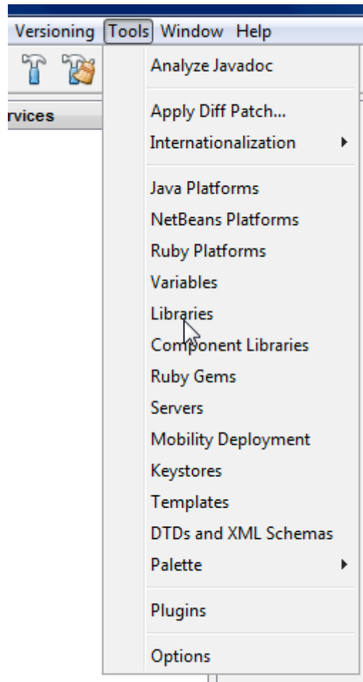
Figure 10-12: Menu Libraries
