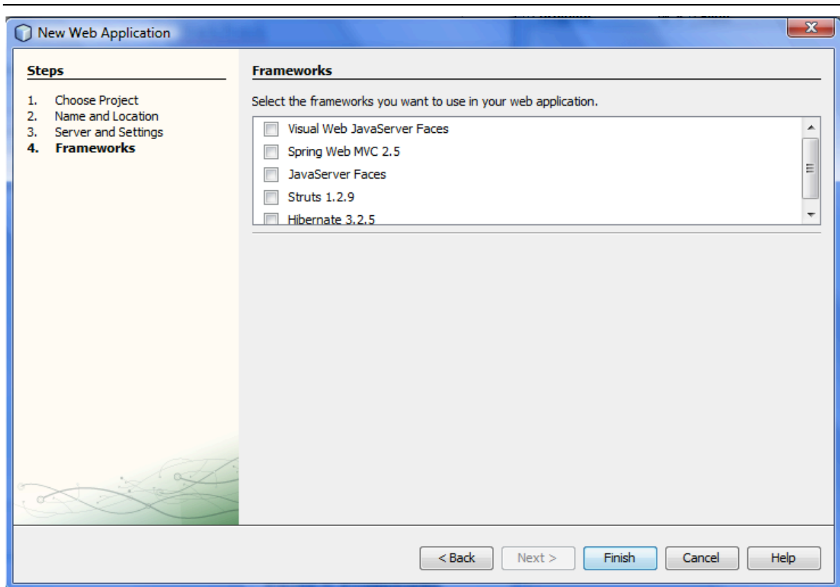
Figure 7-5: Frameworks
