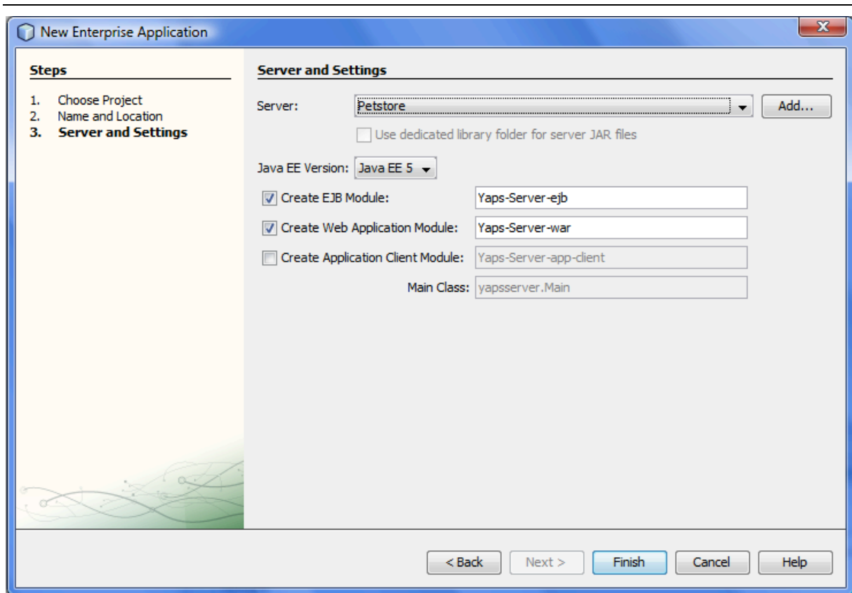
Figure 9-4: Server settings
