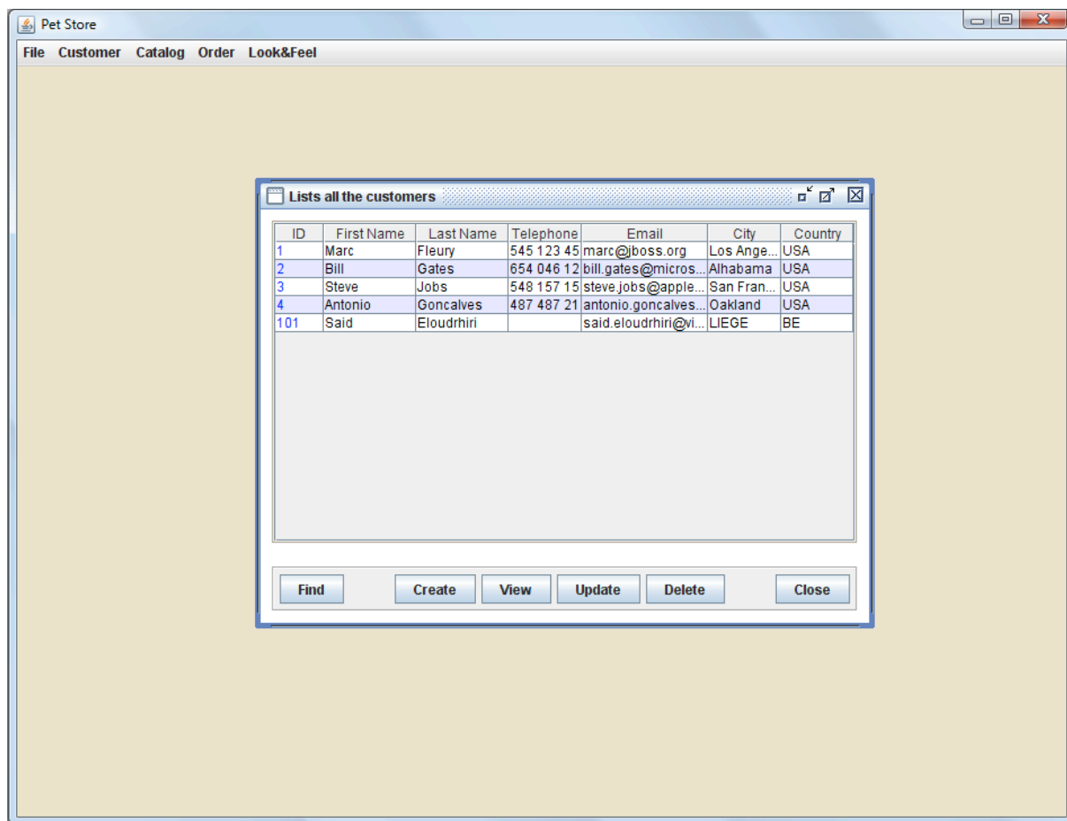
Figure 10-30: Application Yaps-Client
