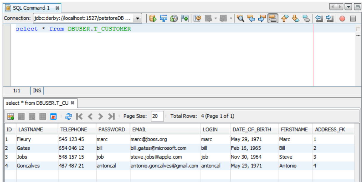
Figure 9-38: Contenu de la table "CUSTOMER"
