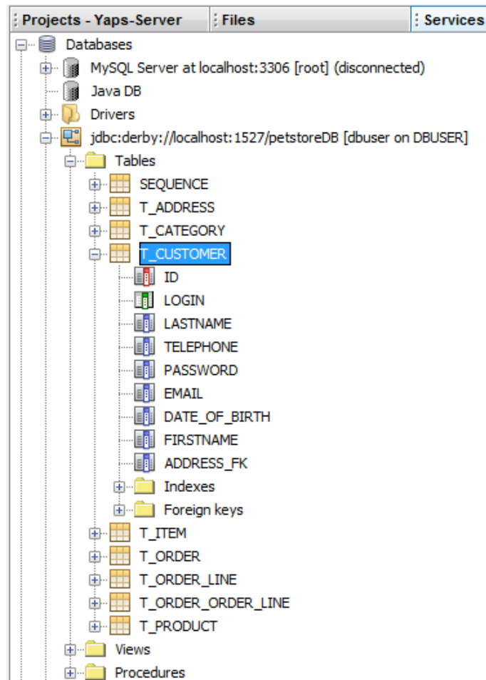
Figure 9-33: Structure de petstoreDB
