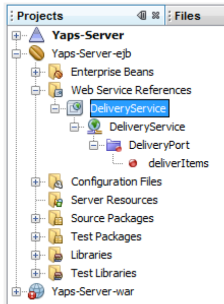
Figure 9-11: Proxy client de DeliveryService
