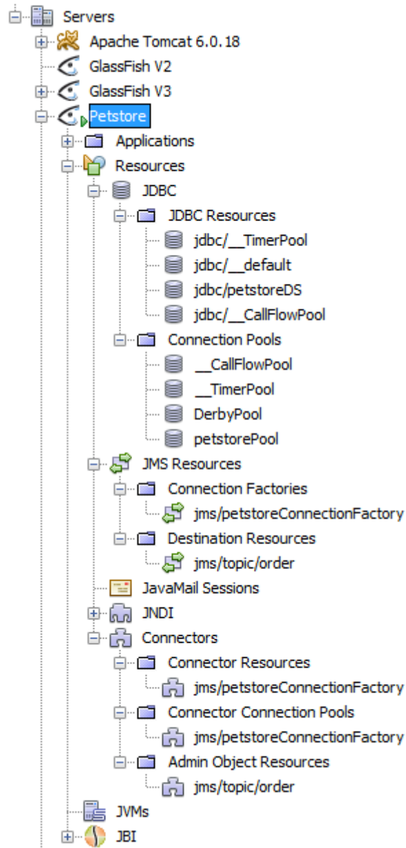
Figure 6-11: Exploration du serveur Petstore
