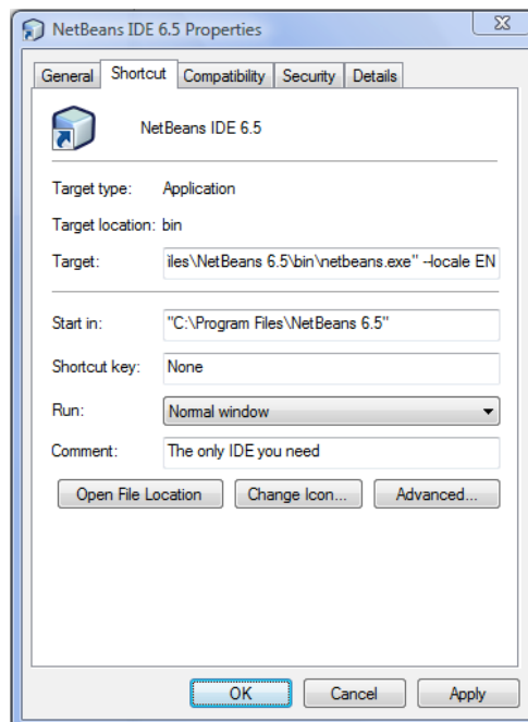
Figure 3-15: Code langue
