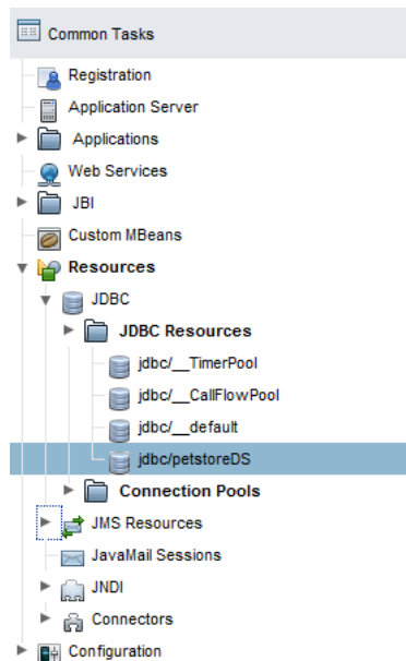
Figure 5-7: JDBC Resources
