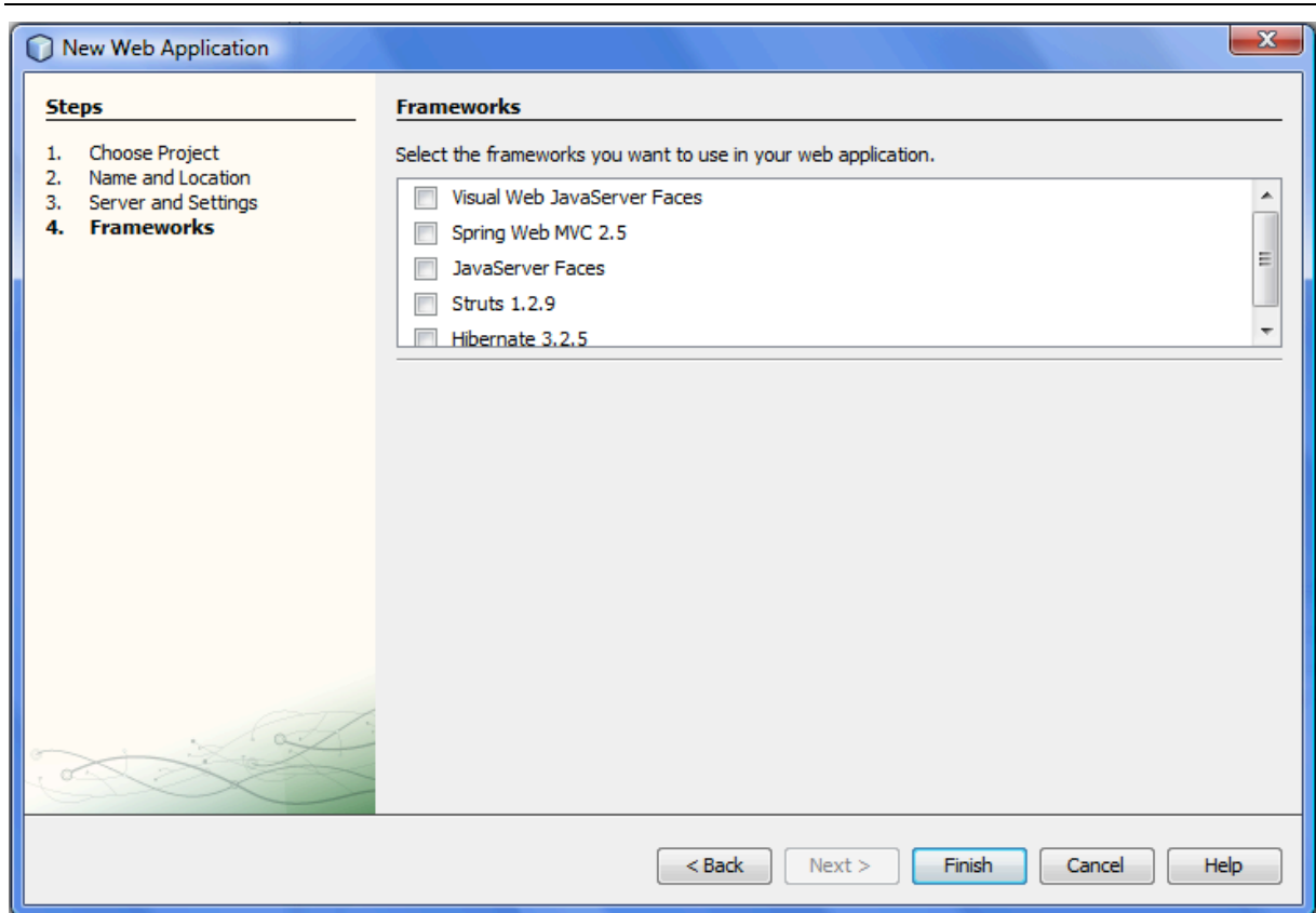
Figure 8-5: Frameworks
