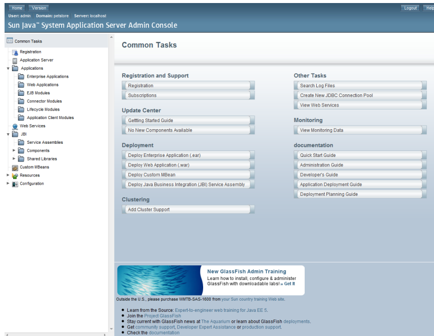
Figure 5-2: Console d'administration
