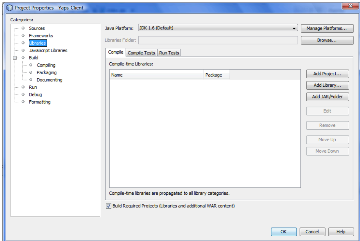
Figure 10-7: Librairies
